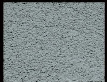
JADEITE
