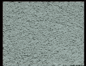
KYANITE
