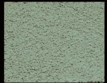
PECTOLITE
