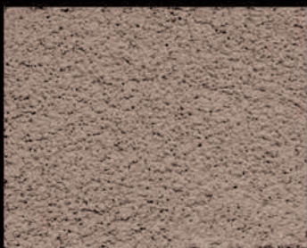
QUARTZ
